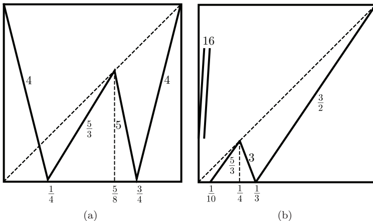
FIGURE 2. Figure (a) shows the graph of the asymmetric W-map of Example 5.3. Figure (b) shows the graph of the map \tau of Example 5.5.
