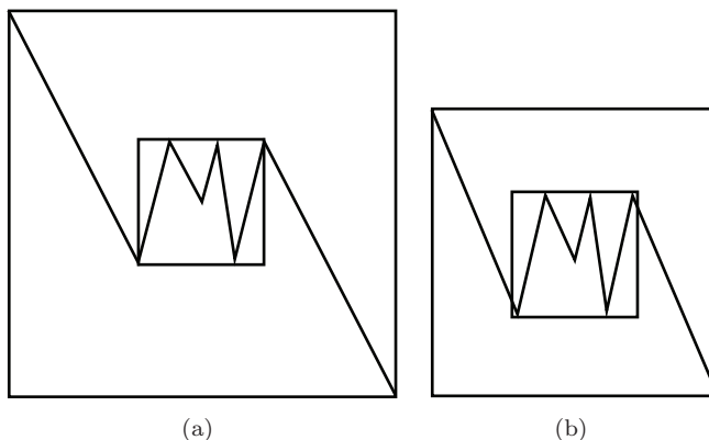
FIGURE 4. Figure (a) shows the graph of \hat{\tau}_0^3 of Example 5.6. Figure (b) shows the graph of \hat{\tau}_t^3 , for t = 0.05 .
