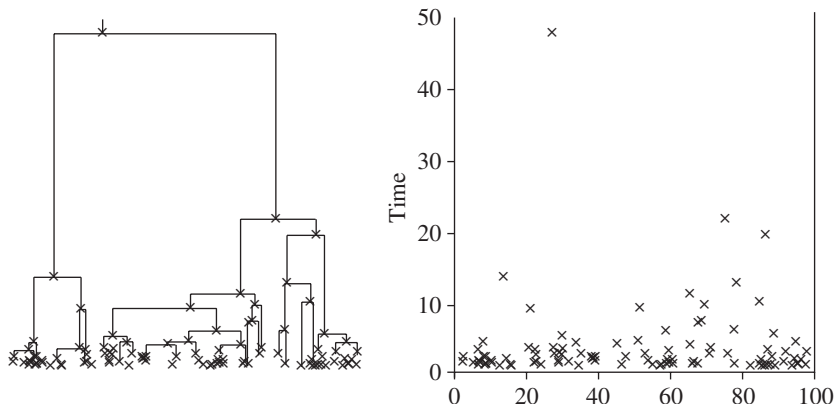
FIGURE 2: The point process \pi_{1,t} (right) represents the lineage tree of a ‘continuum tree’ of species (left).
