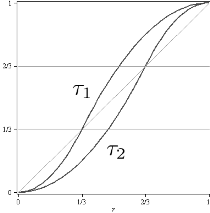
FIGURE 1. Maps \tau_1 and \tau_2 in Example 3.4
