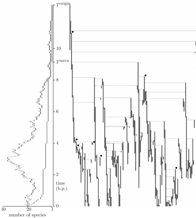
Fig. 6 A realization of c - \text{TREE}_{20} , a complete clade on 20 extant species. The figure is drawn so that each species occupies a vertical line [from time of origin to time of extinction (or present)], different species evenly spaced left-to-right (so that each subclade is a consecutive series), using the convention: daughters are to right of parents, earlier daughters rightmost. On the left are time series: the outer line is total number of species, the inner line is number of ancestors of extant species. Filled circle indicate “new type” species, used later to construct genera. In this realization there were a total number 142 of extinct species, with a maximum of 38 species at one time; T^{\text{mrca}} = 9.05 and T^{\text{origin}} = 12.75
