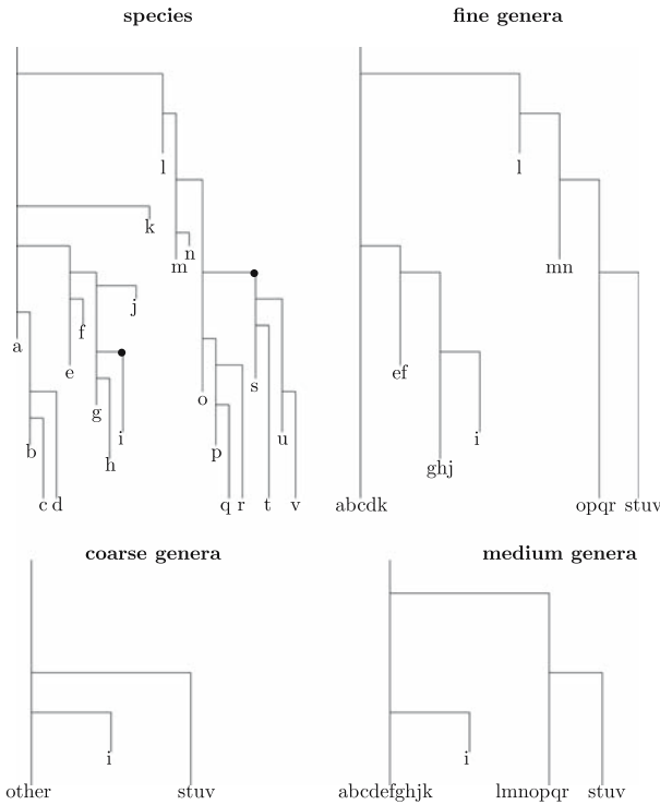
Fig. 1 Illustration of our schemes for defining genera in terms of new types. Above left is a complete clade of 6 extant and 16 extinct species ( abcd...uv ), with two species \{i, s\} designated as new types and marked by filled circle . In the fine scheme, this induces eight genera (three extant), whose tree is shown above right . The other schemes are shown below , with compressed time scale
