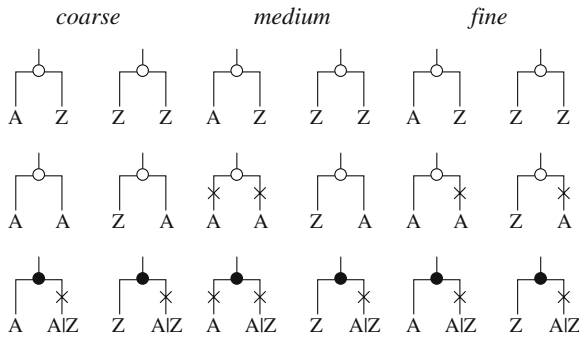
Fig. 9 Catalog of rules for assigning marks cross symbol in the three classification schemes. The figure shows a branchpoint in a phylogenetic tree redrawn as lineage segments. Daughter lineage on right . Filled circles indicate daughter is “new type”. Z or A indicate zero or non-zero number of new type species in subclade. A|Z stands for “A or Z”
