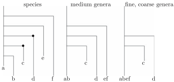
Fig. 5 An atypical tree and its genera. There are two “new type” species, \{c, d\} . Note that the coarse/fine genus \{abef\} is paraphyletic while the medium genus \{ef\} is not
