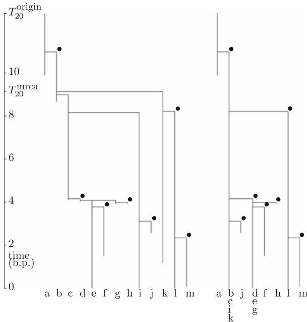
Fig. 8 The phylogenetic trees on medium genera ( left ) and coarse genera ( right ) corresponding to the fine genera in Fig. 7. There are 13 medium and 8 coarse genera
