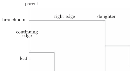
Fig. 1 Illustration of our schemes for defining genera in terms of new types. Above left is a complete clade of 6 extant and 16 extinct species ( abcd...uv ), with two species \{i, s\} designated as new types and marked by filled circle . In the fine scheme, this induces eight genera (three extant), whose tree is shown above right . The other schemes are shown below , with compressed time scale
